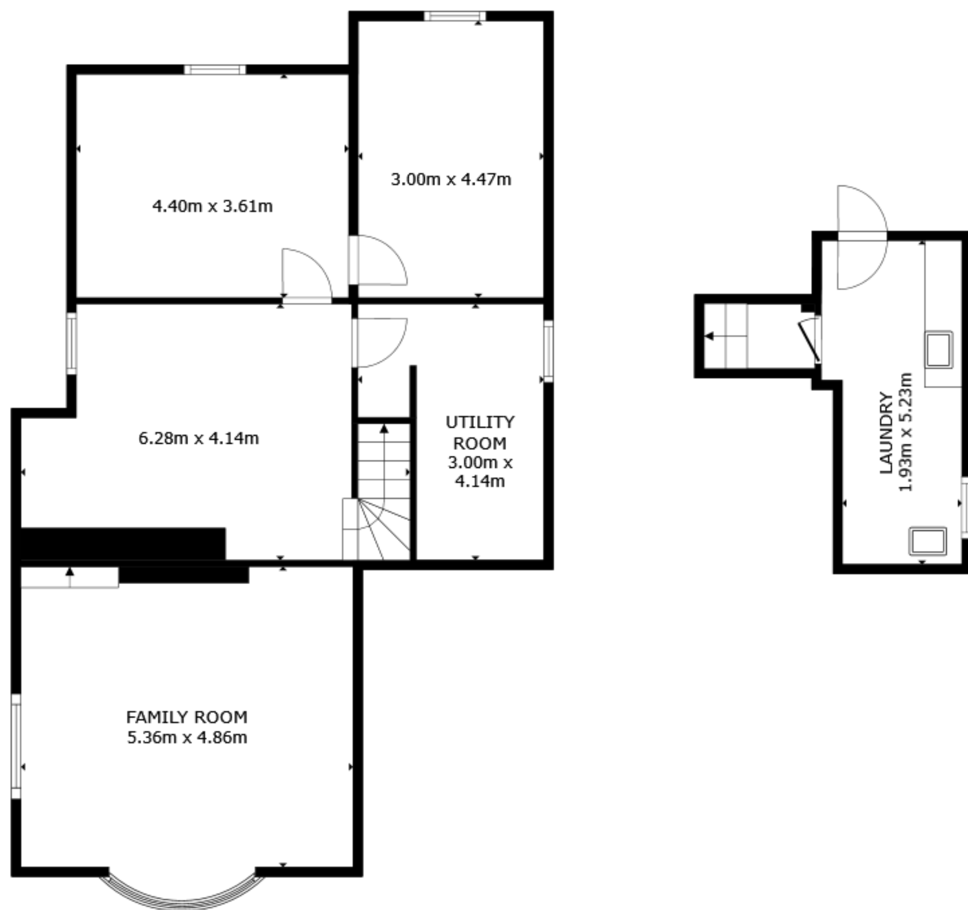
FLOOR 1
