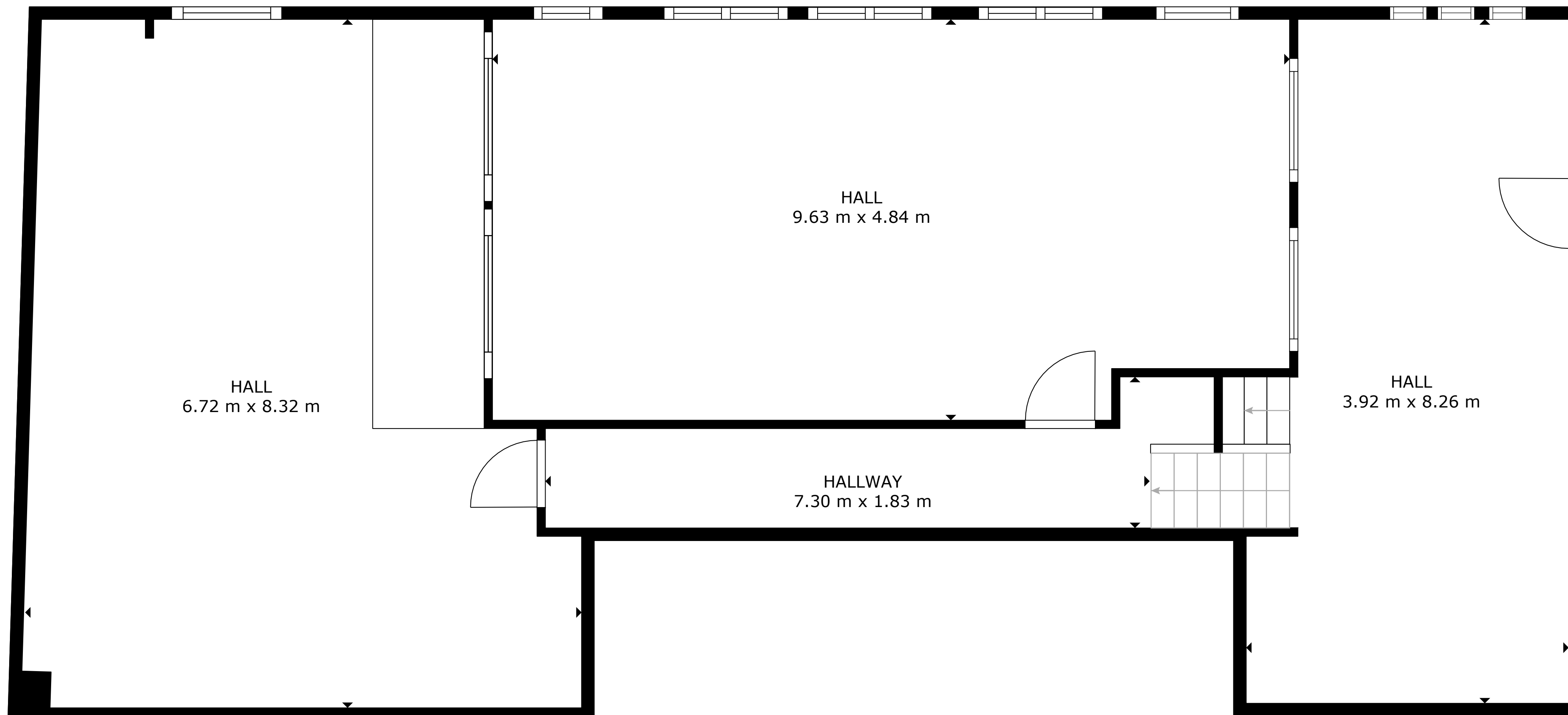
FLOOR 1
