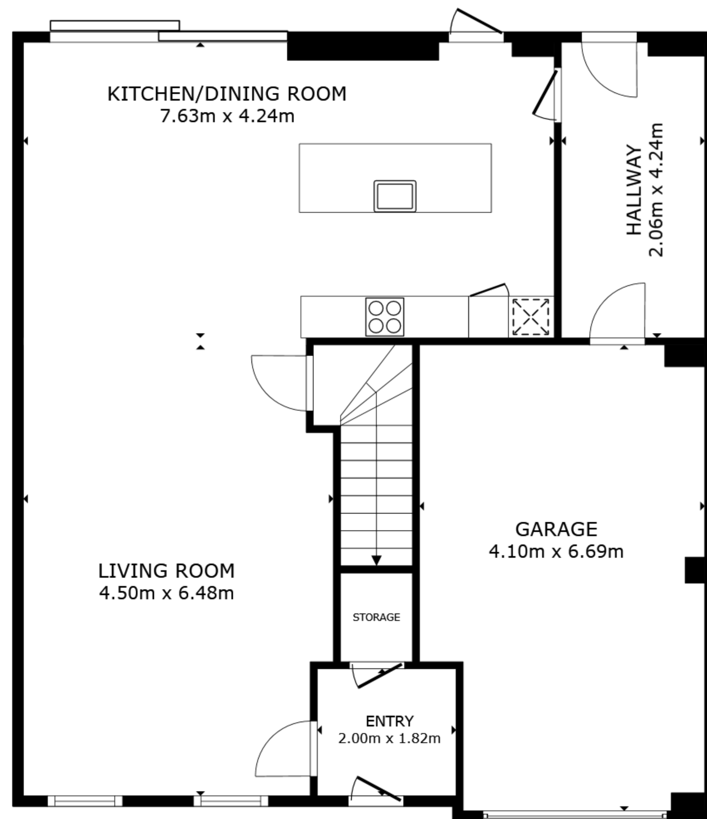
FLOOR 1
