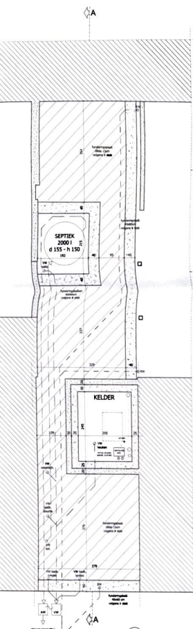
DERING- / RIOLERINGPLAN
