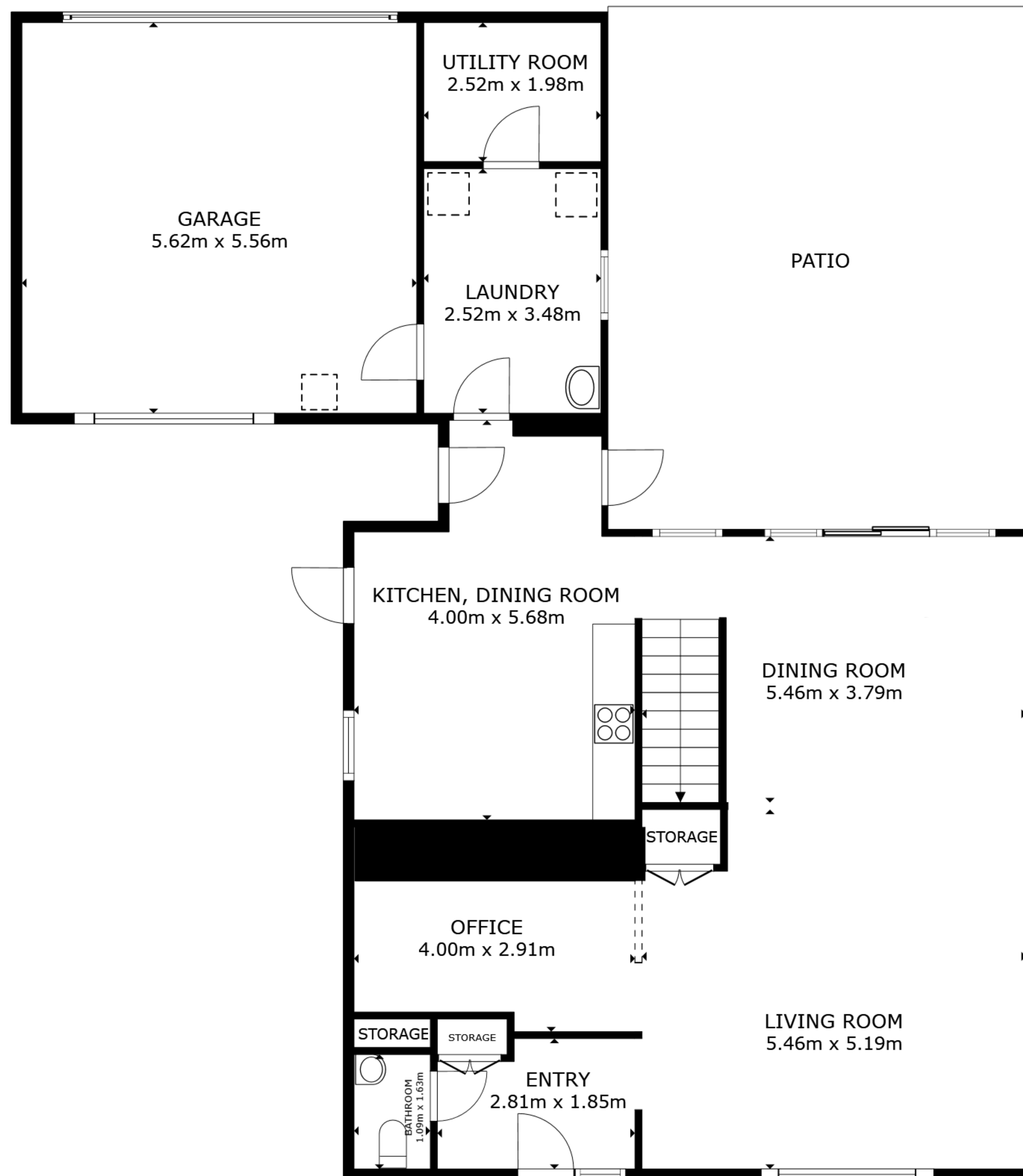
FLOOR 1
