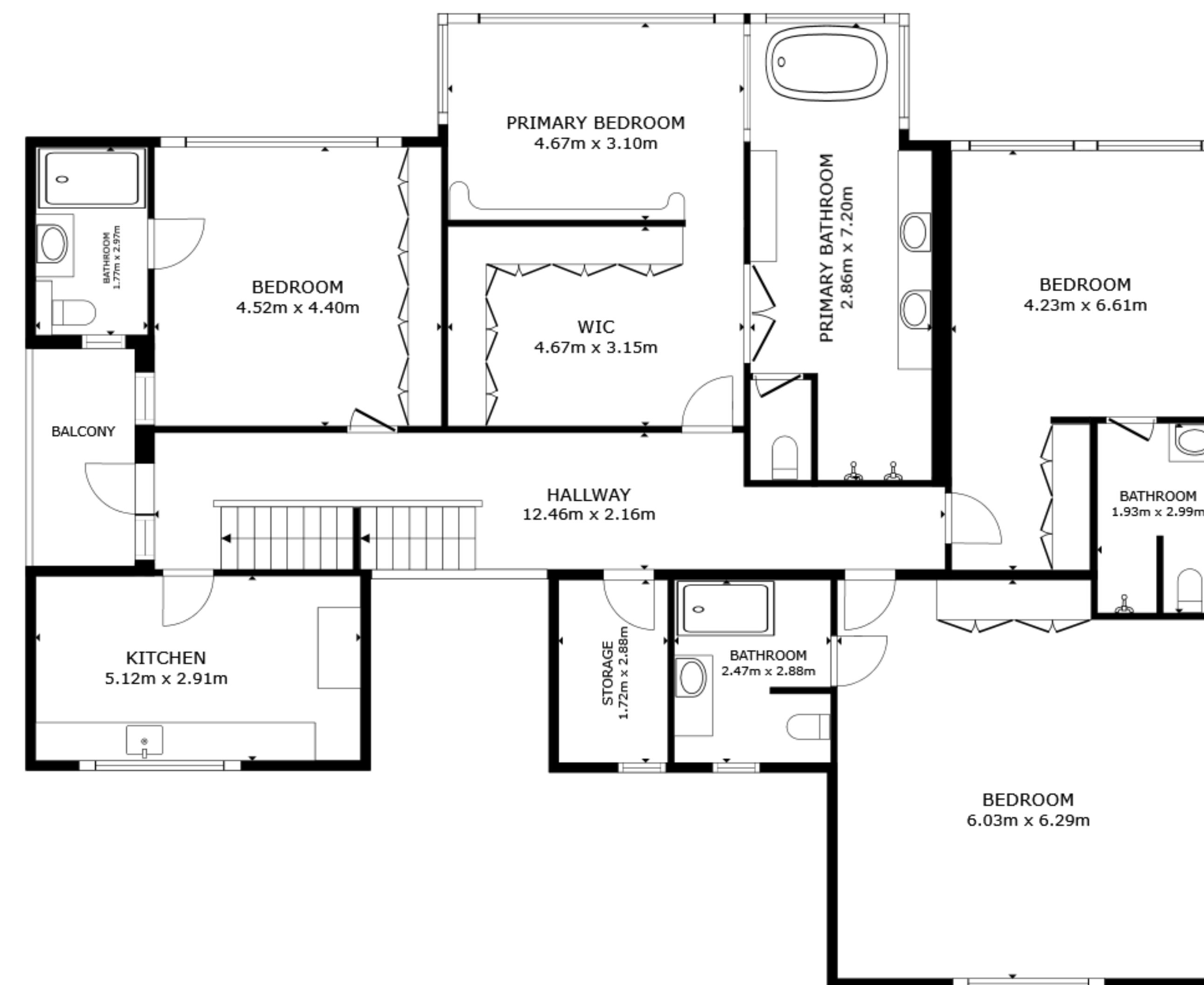
FLOOR 2
