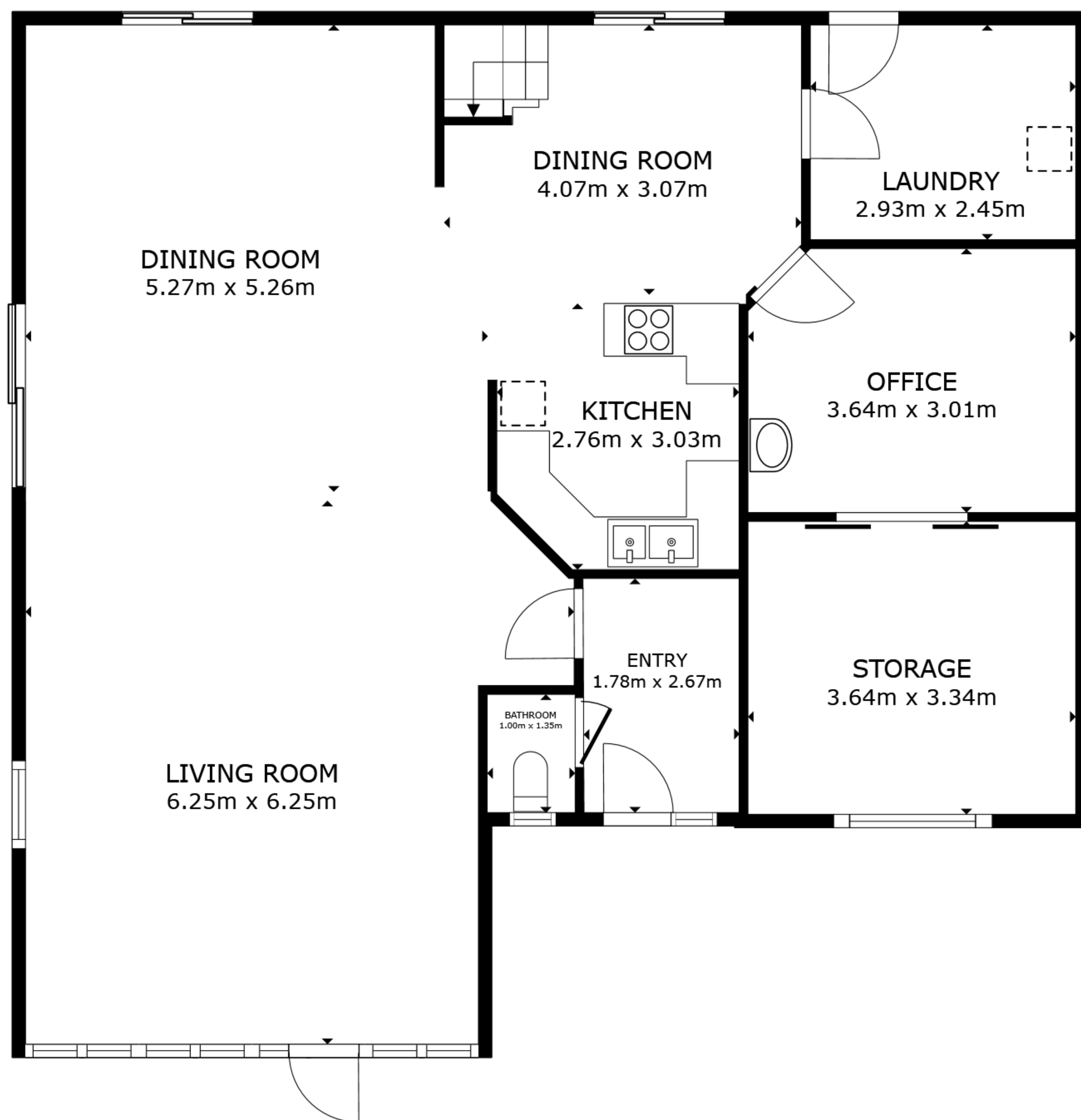
FLOOR 1
