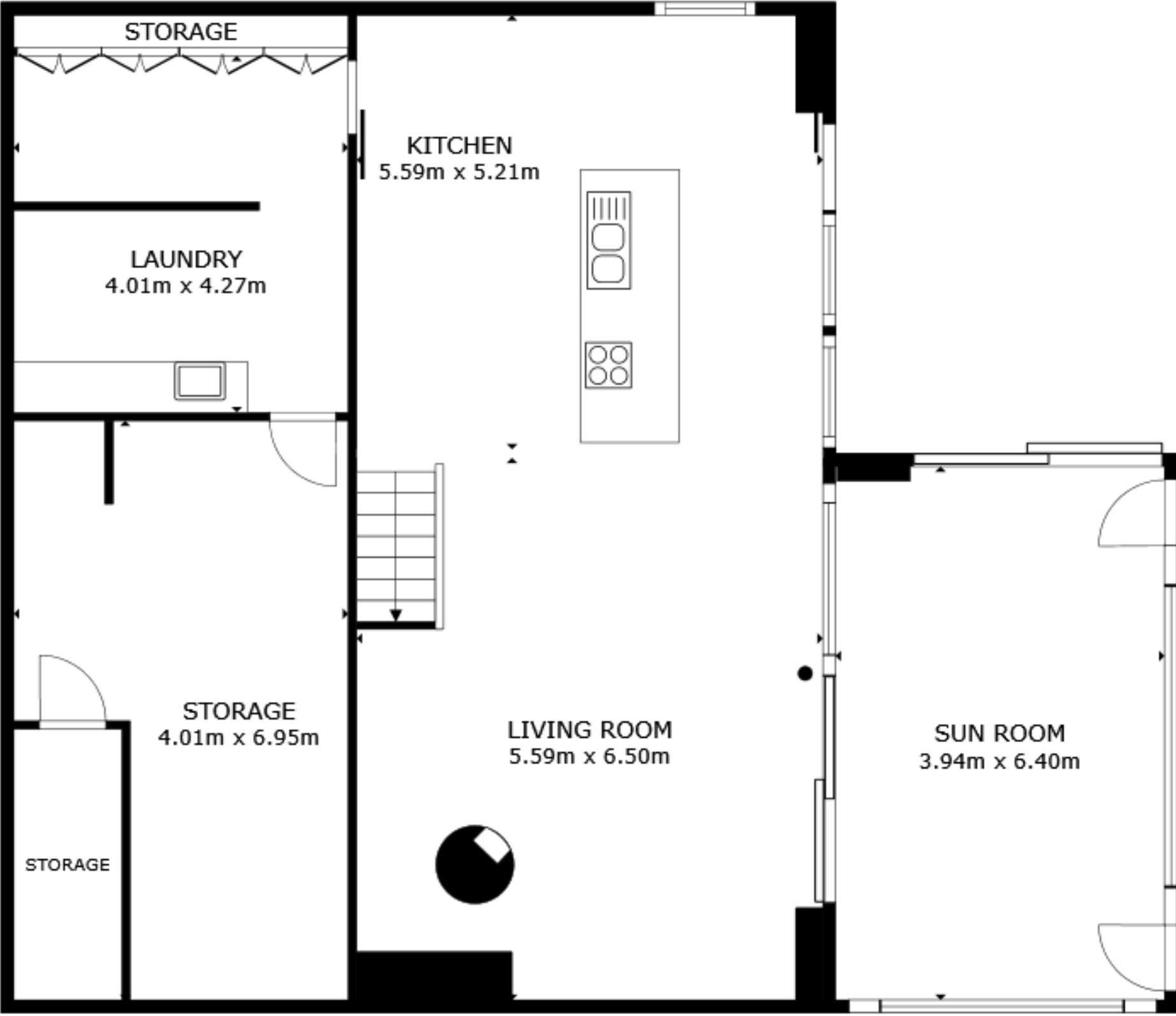
FLOOR 1
