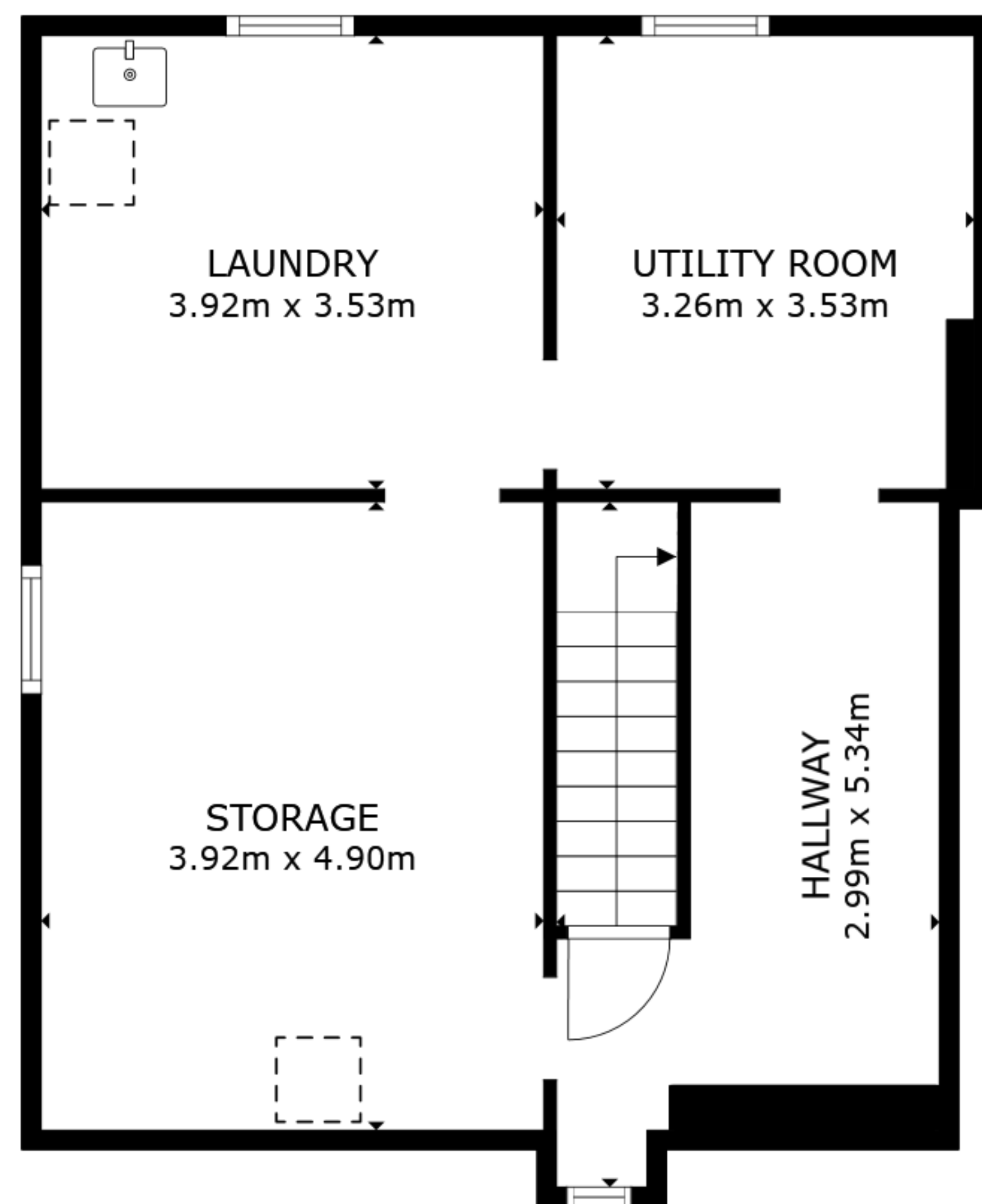
FLOOR 1
