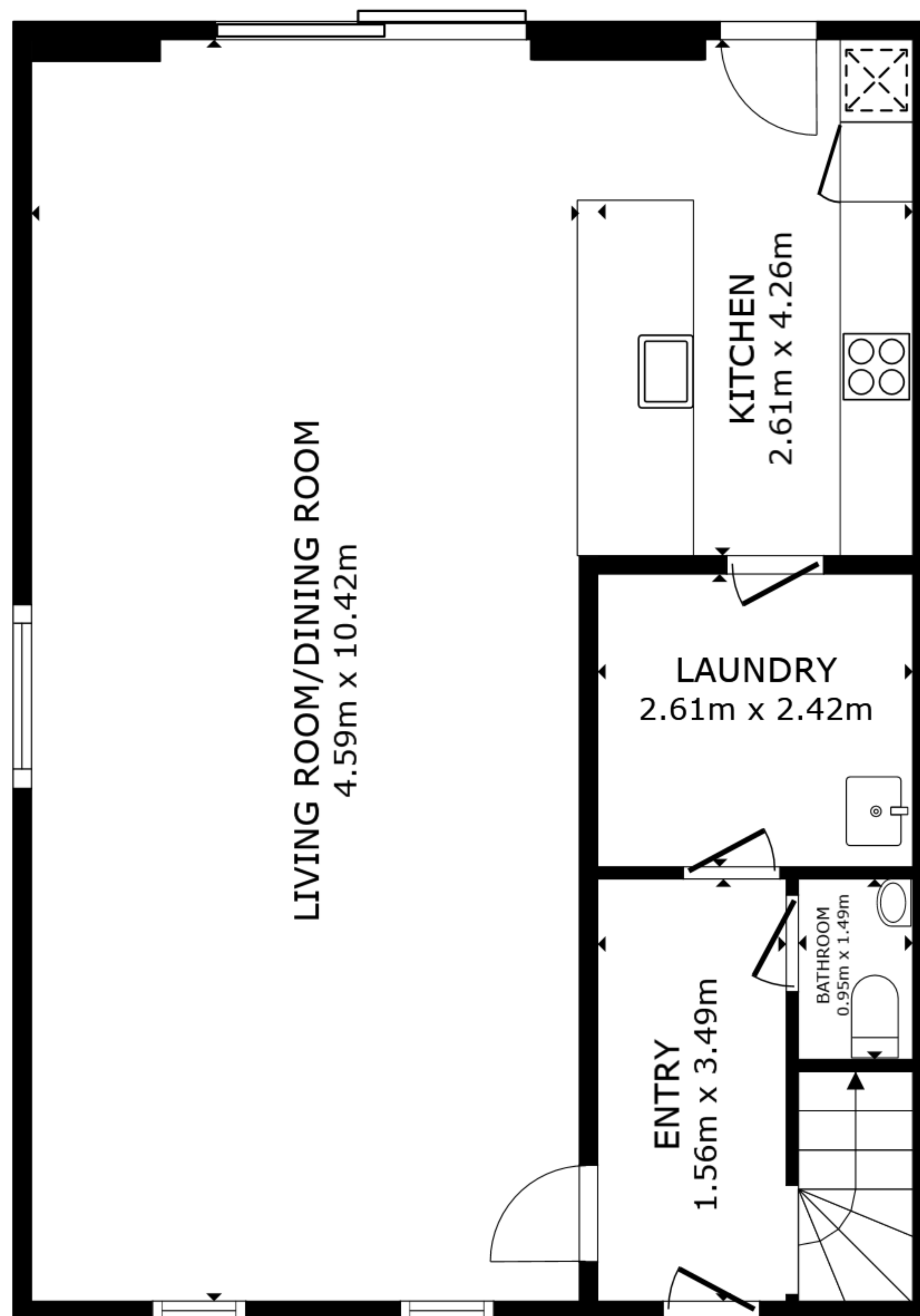
FLOOR 1
