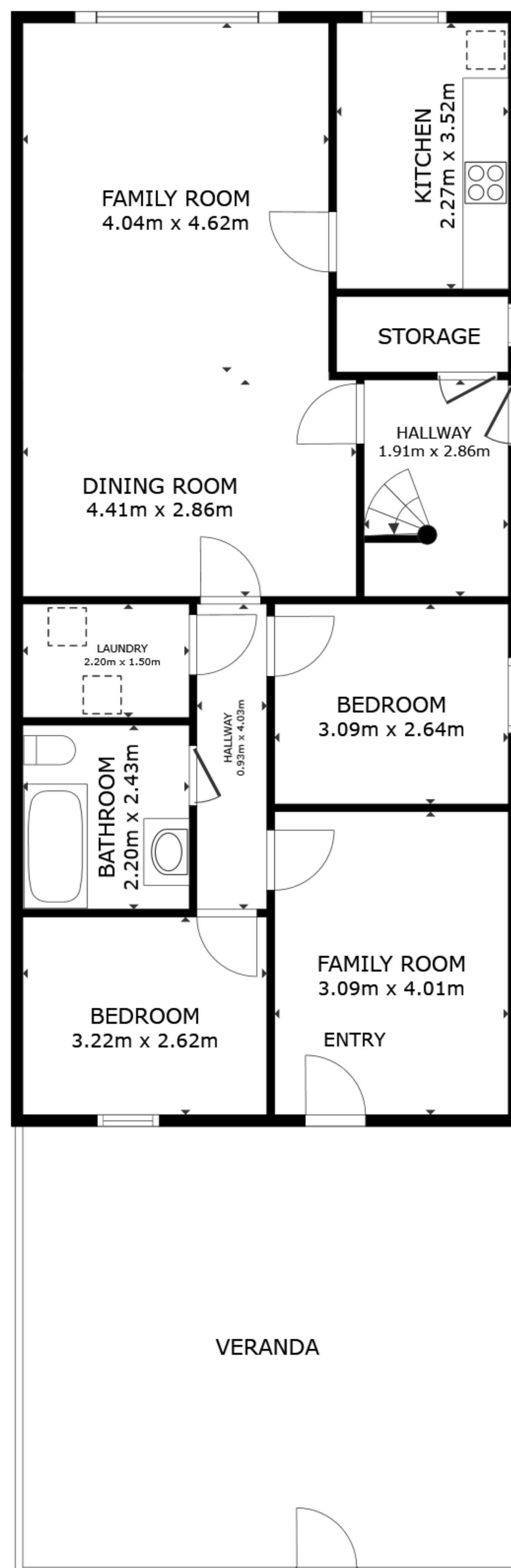
FLOOR 1
