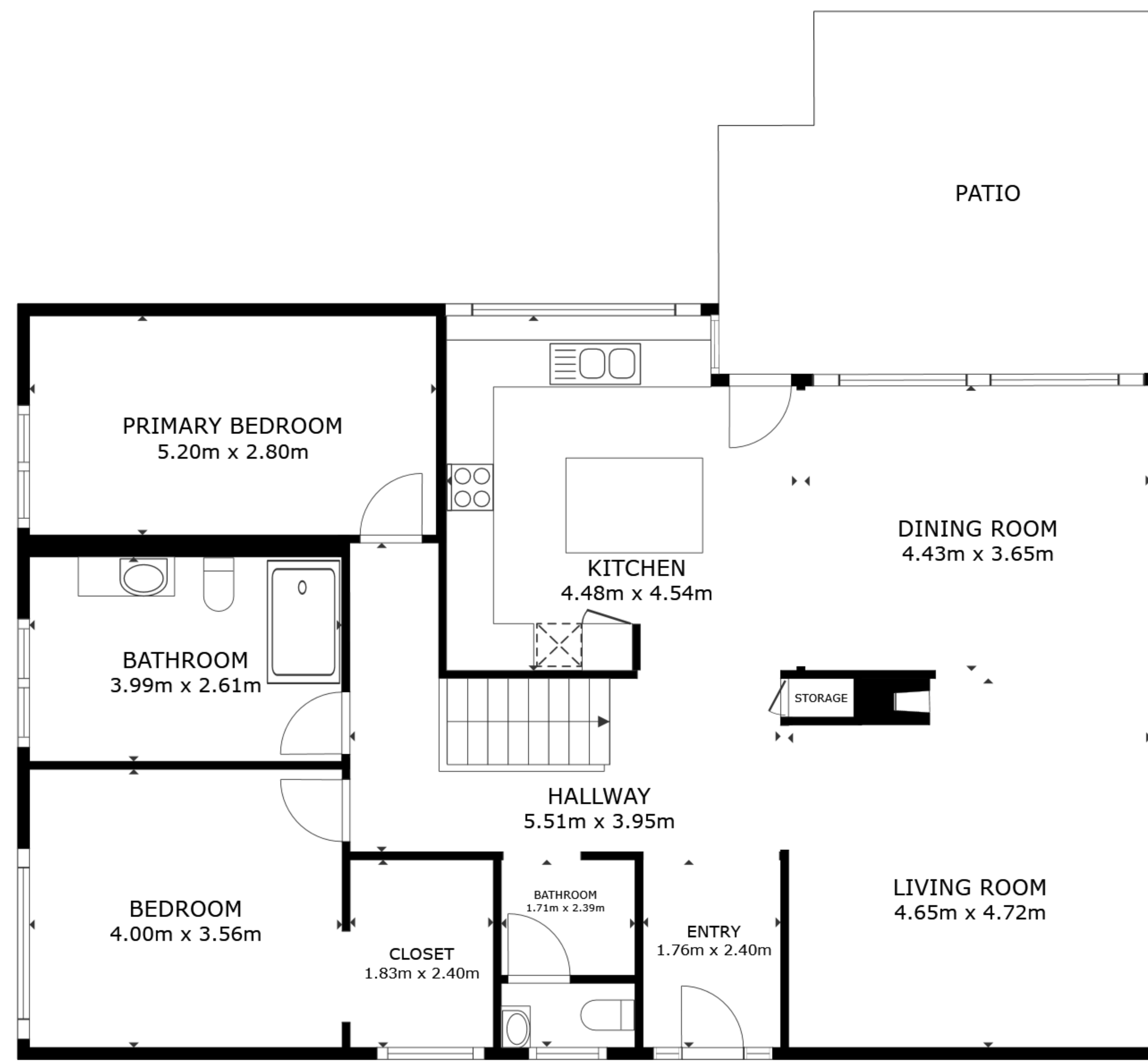
FLOOR 2
