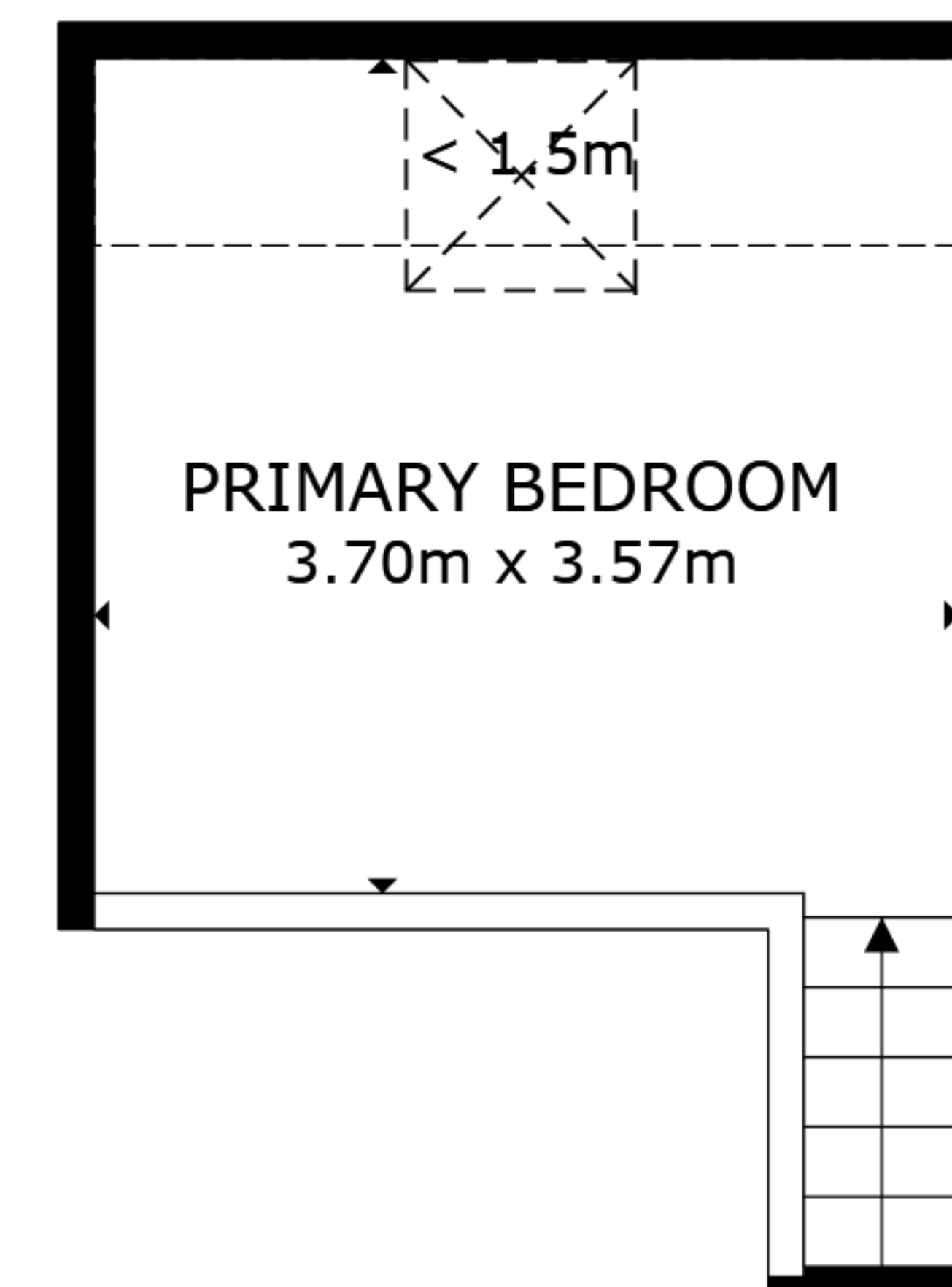
FLOOR 4
