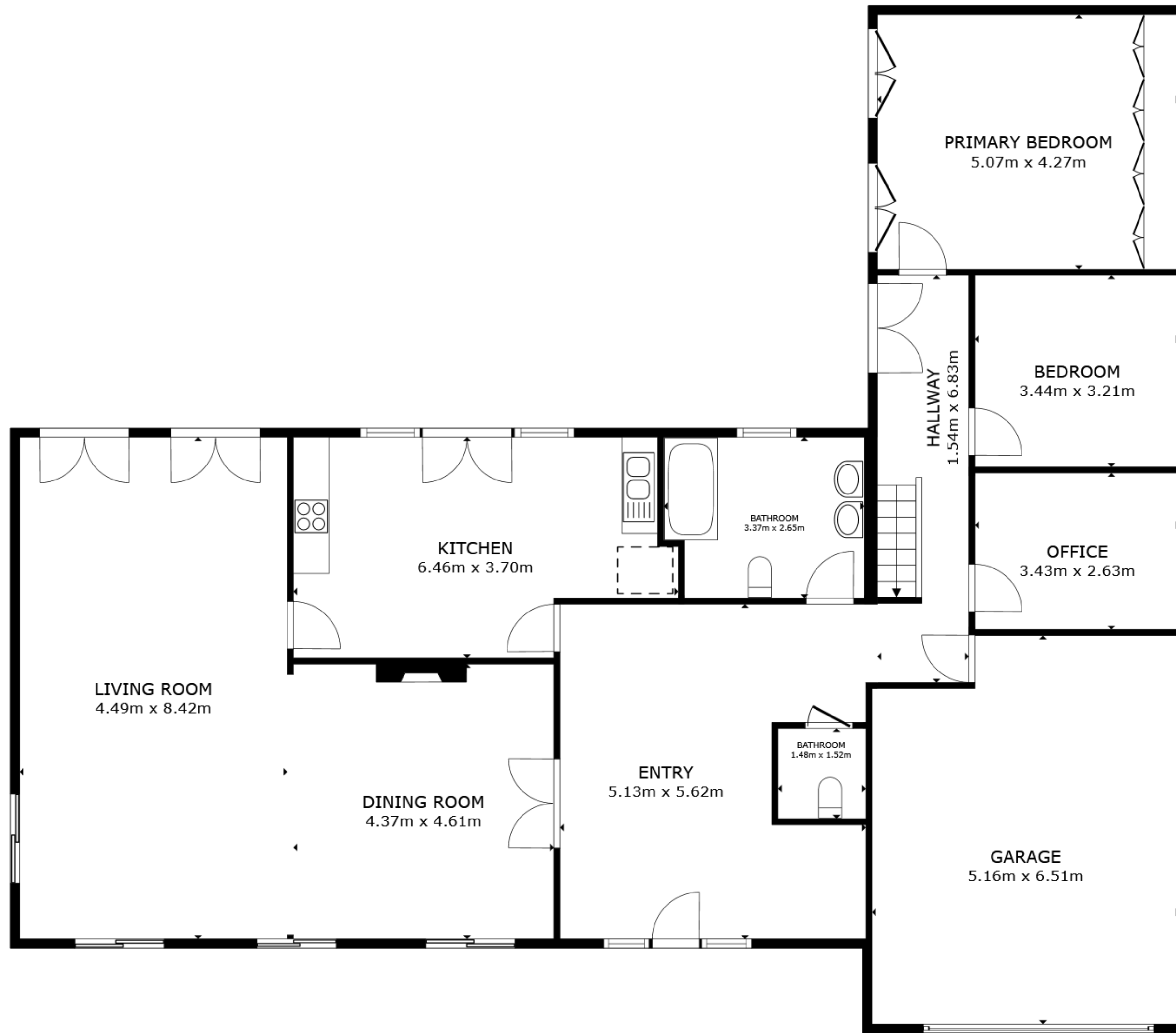
FLOOR 1
