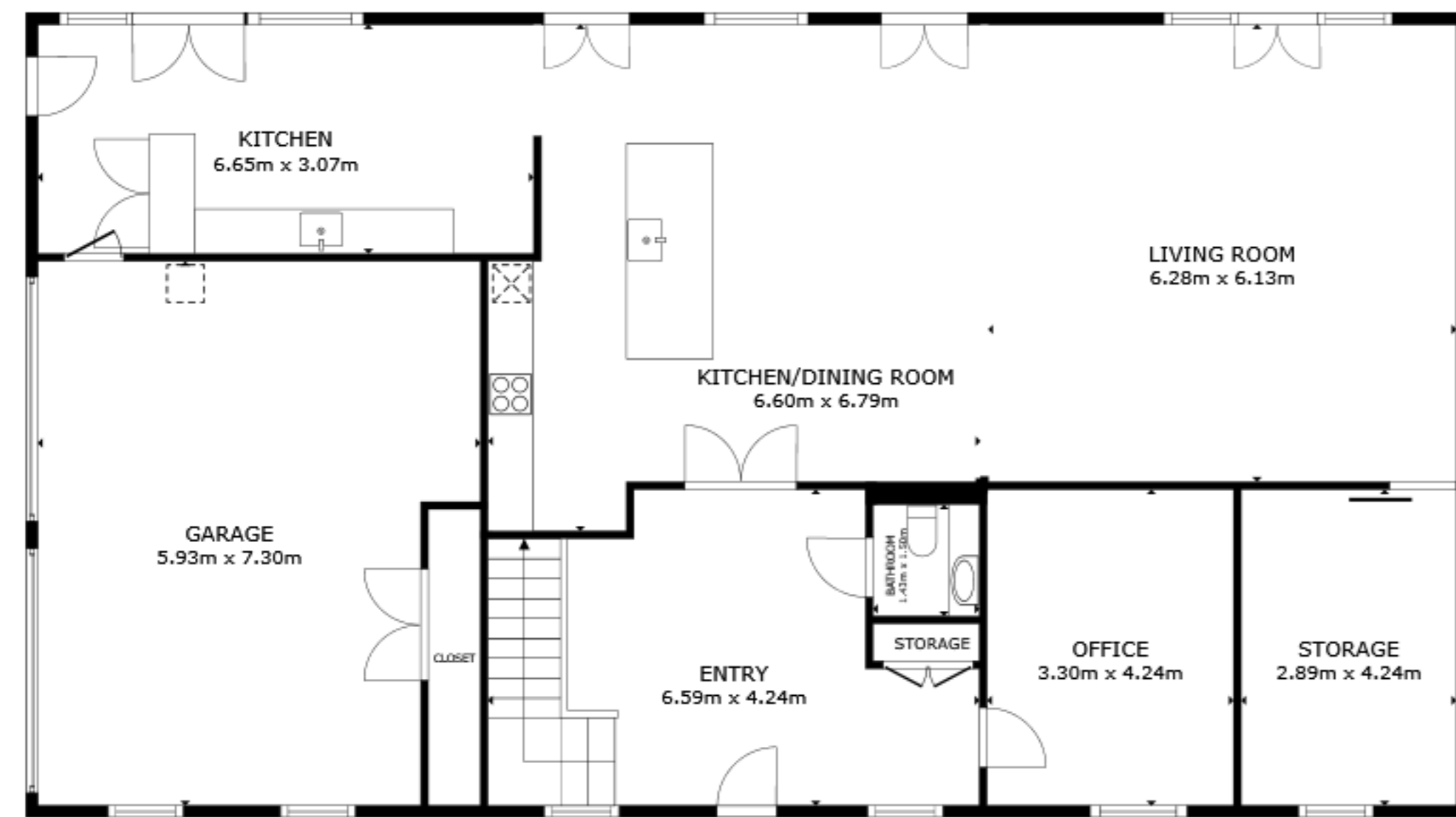
FLOOR 1
