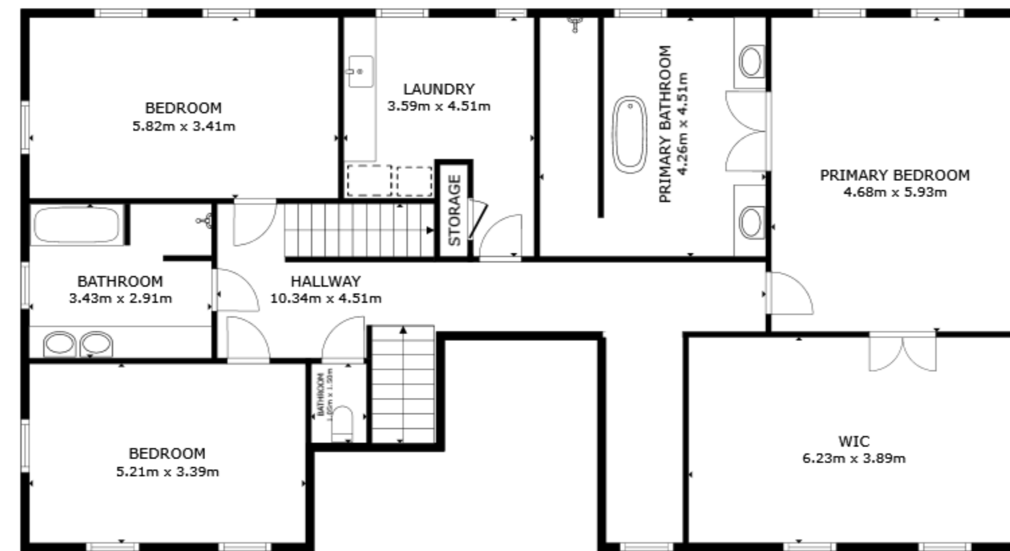
FLOOR 2
