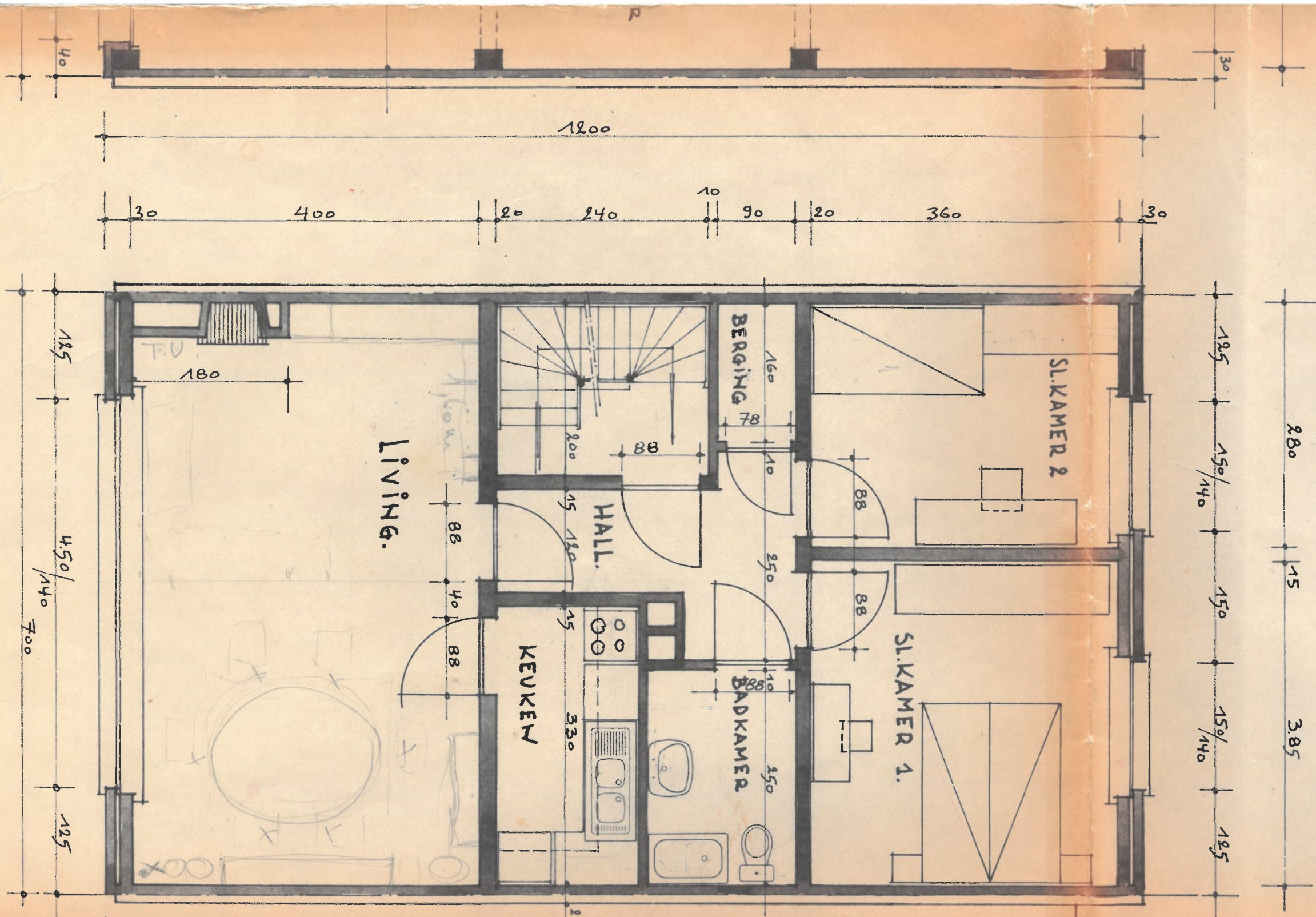
PLAN 1 ste VERDIEPING.
