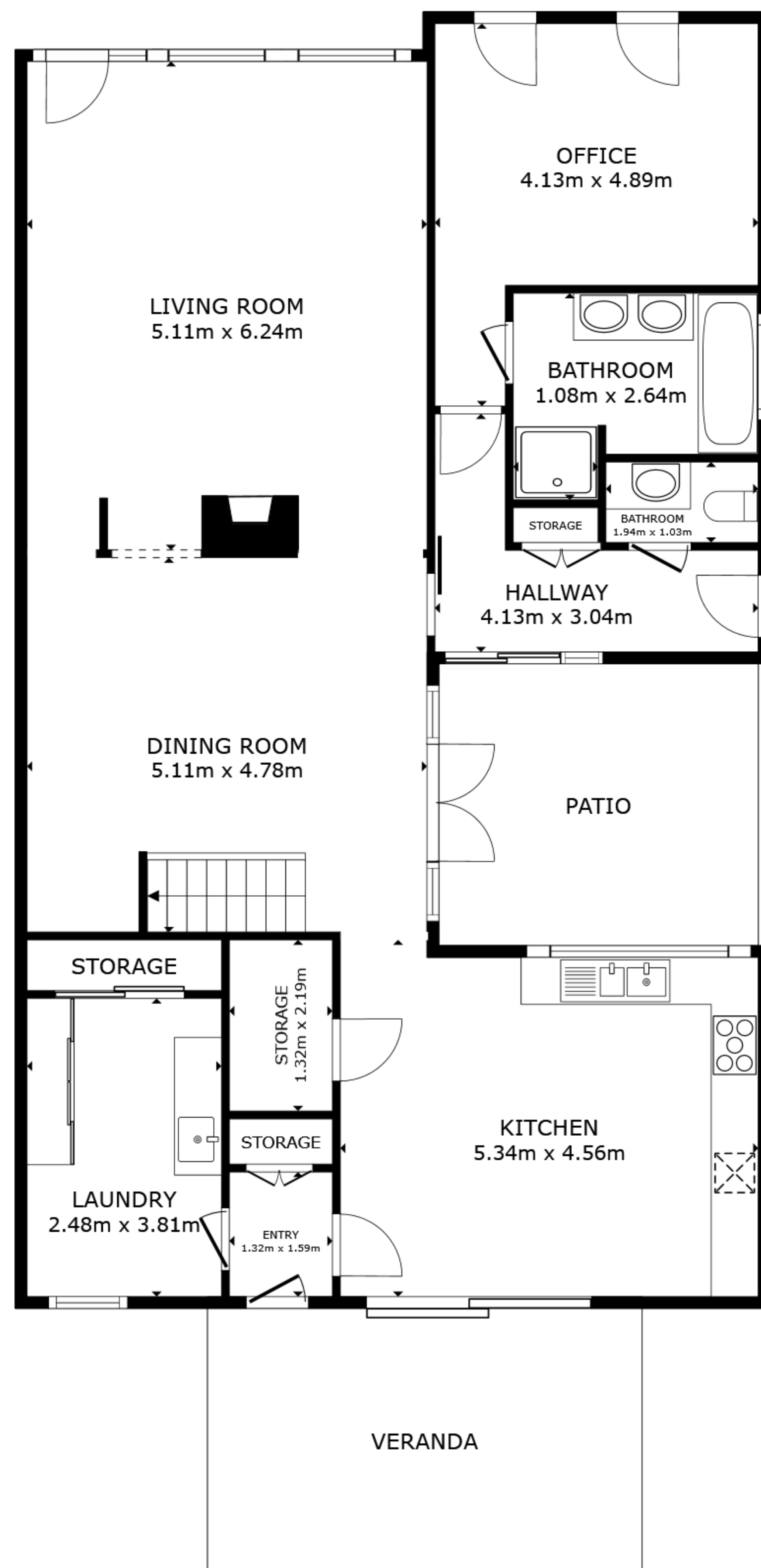
FLOOR 1
