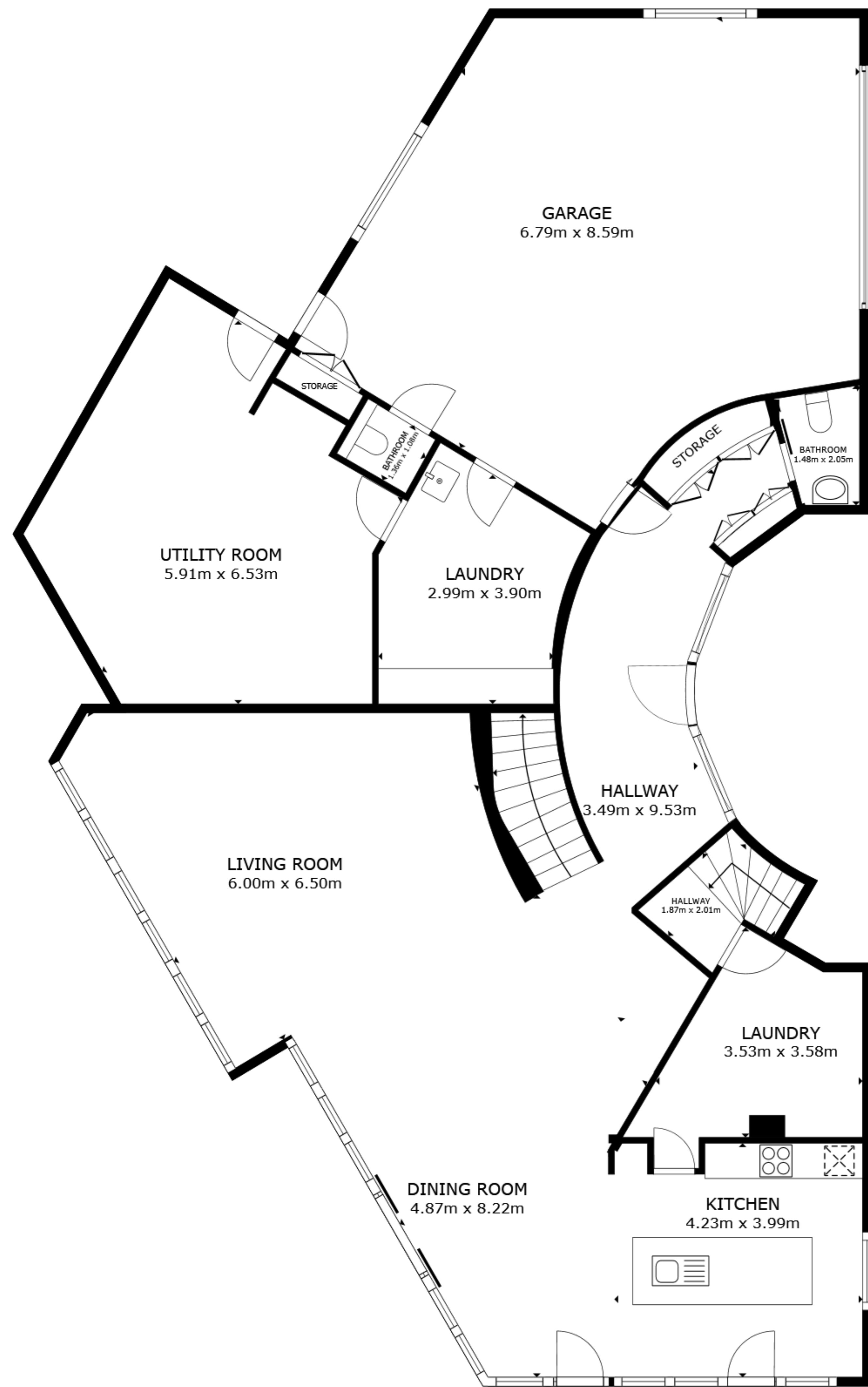
FLOOR 1
