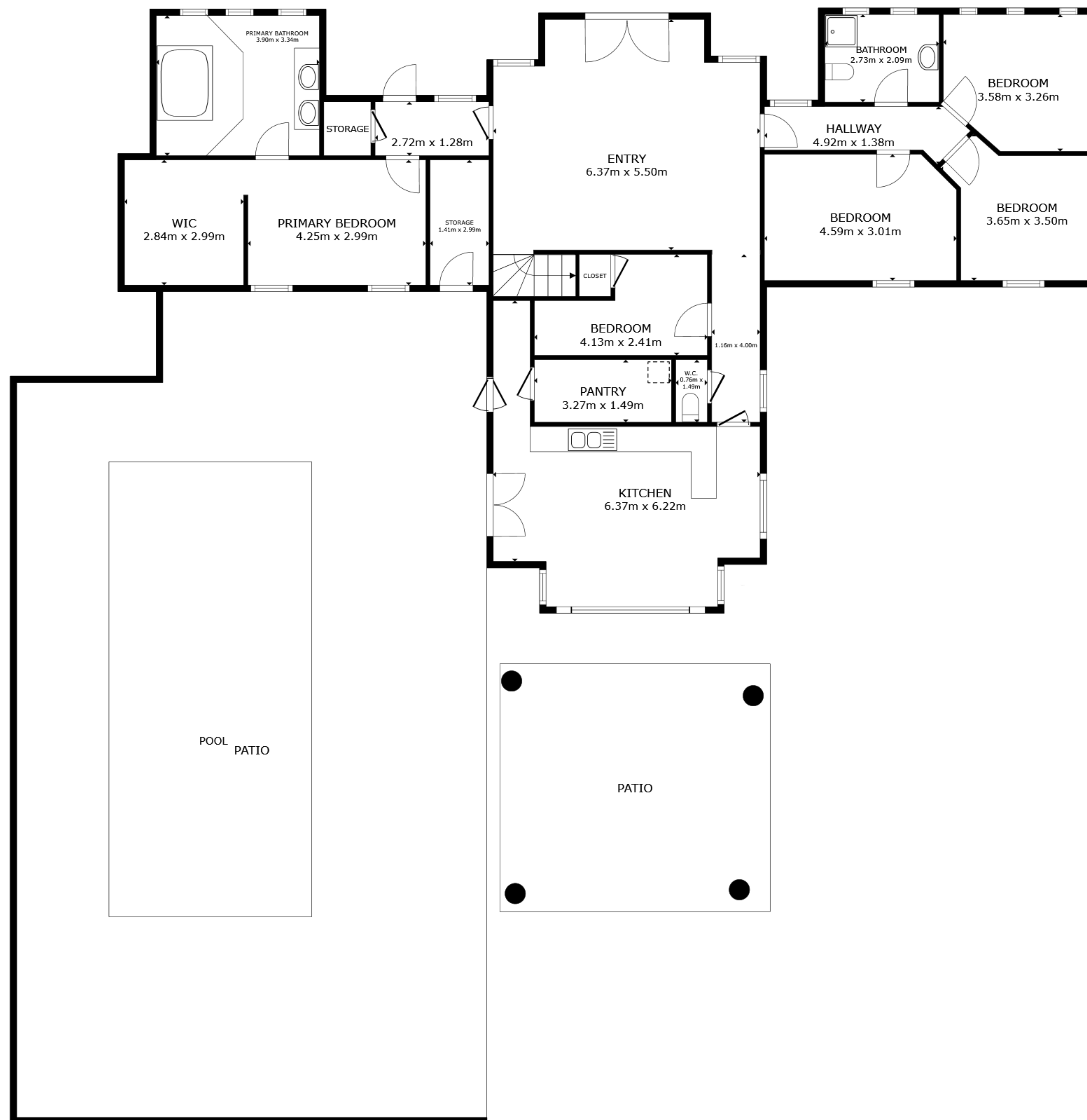
FLOOR 1
