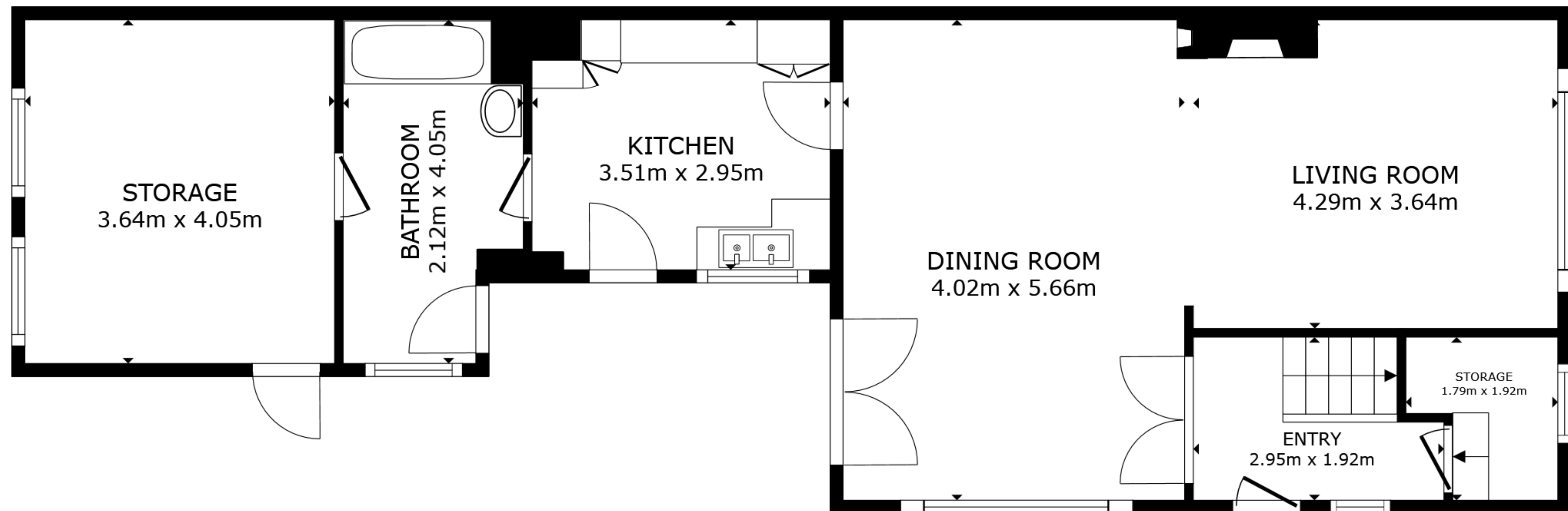
FLOOR 1
