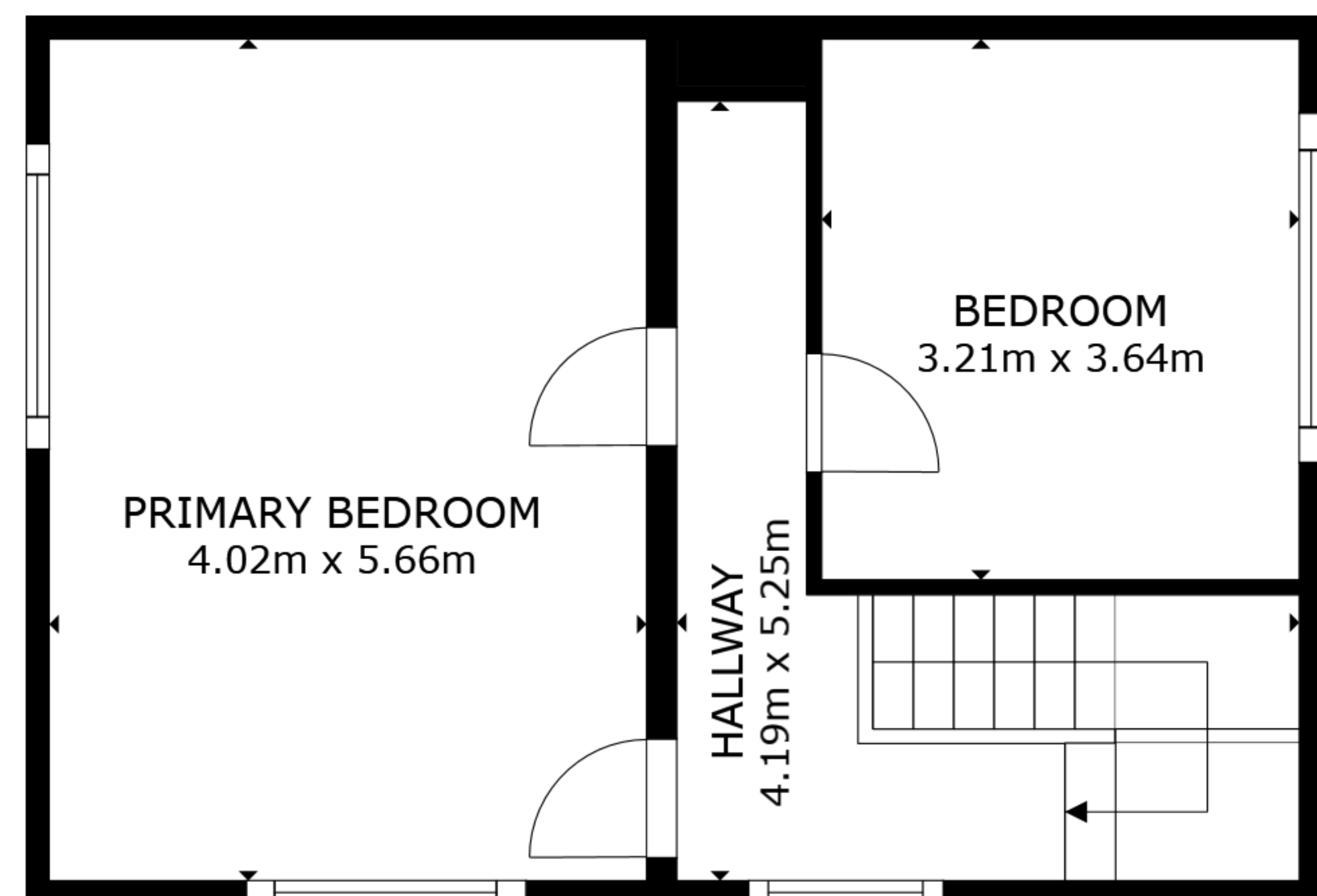
FLOOR 2
