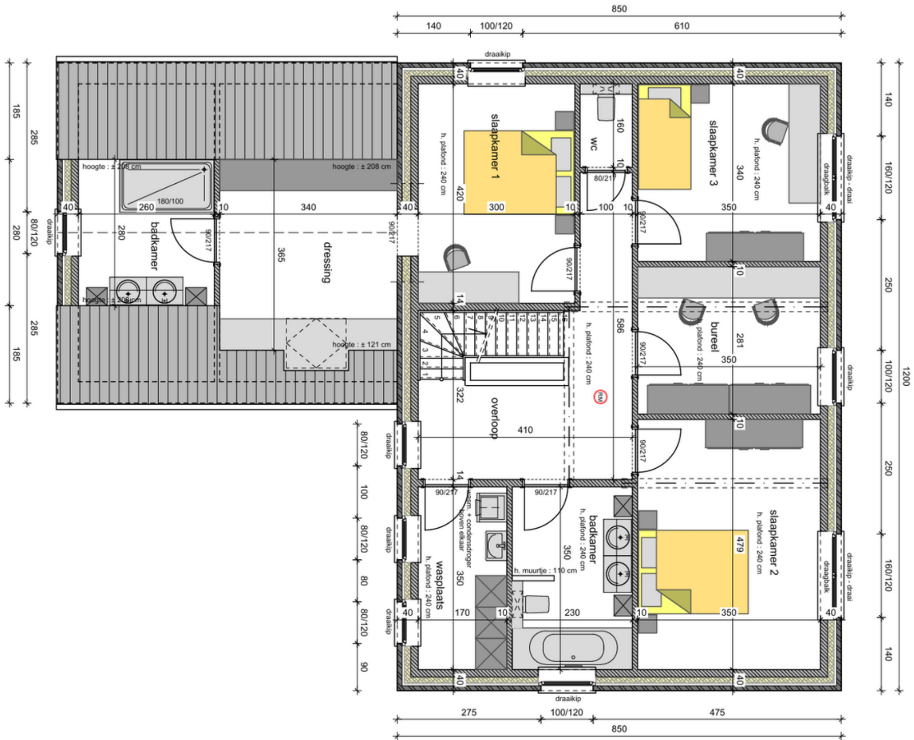
plan verdieping
