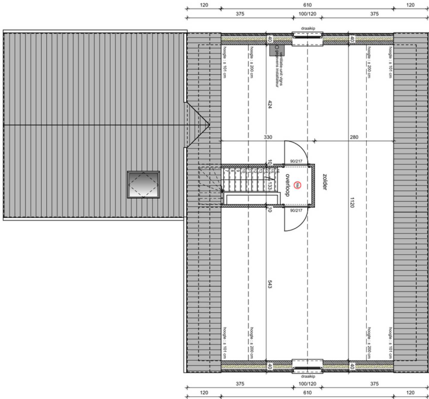
plan zolder
